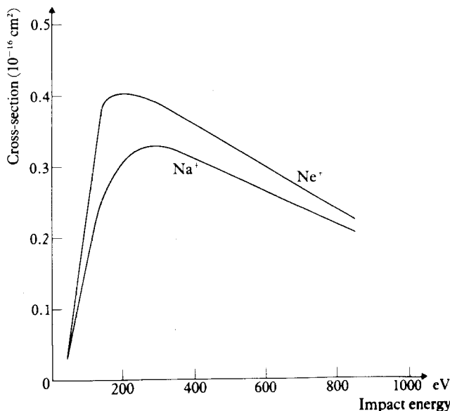
12.7 The cross-section for ionisation of Na^+ and Ne^+ by electron impact.
